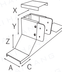
Side opening 扭向槽口短蓋
