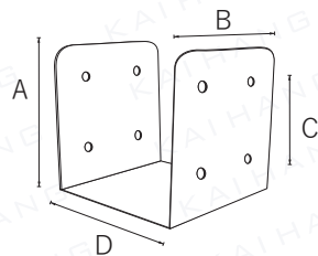
U-shaped connector U 型槽駁片
