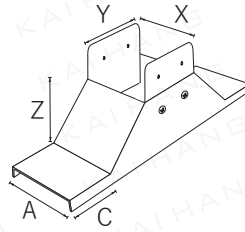
Top opening 90° 槽蓋刁士
