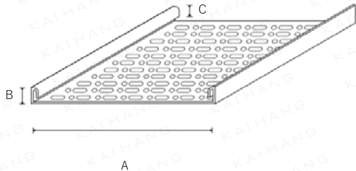
Without built-in connector 普通平邊款
