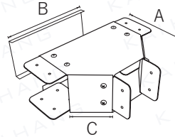
Top opening-Type 2 頂開蓋型-款式2
