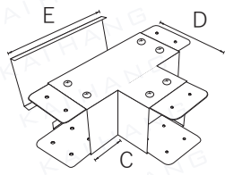
Top opening-Type 1 頂開蓋型-款式1
